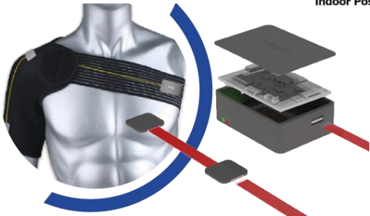
Indoor Positioning
