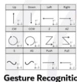
Gesture Recognition
