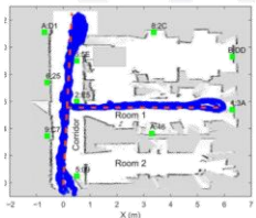
Indoor Positioning
